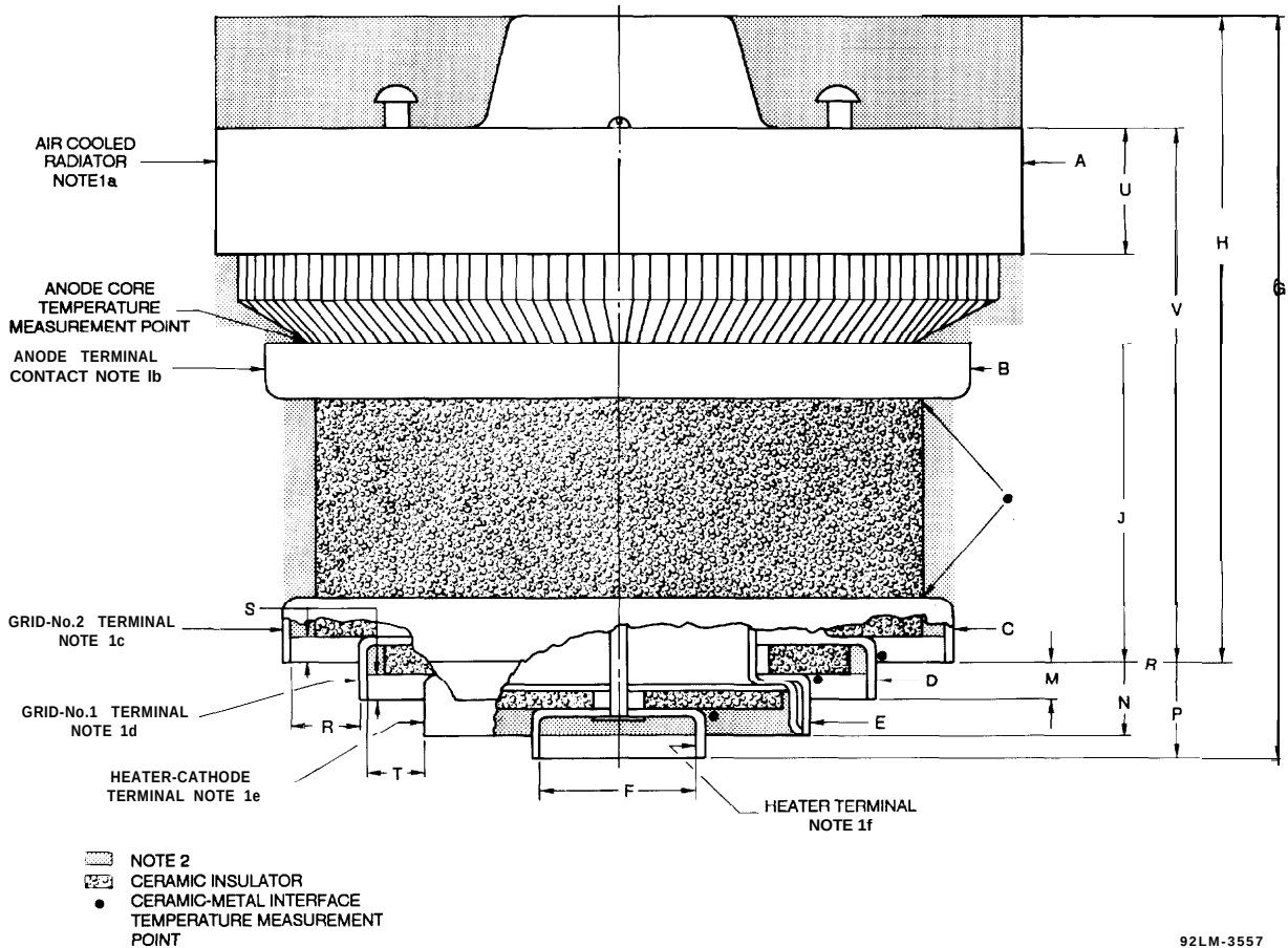
Figure 7 - Dimensional Outline
