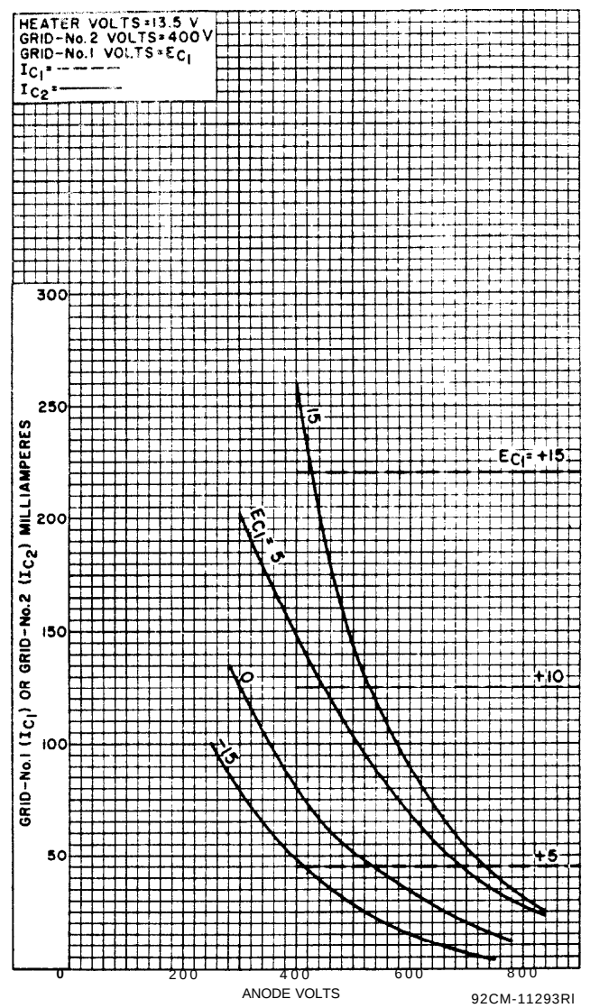
Figure 4 - Typical Grid Characteristics
